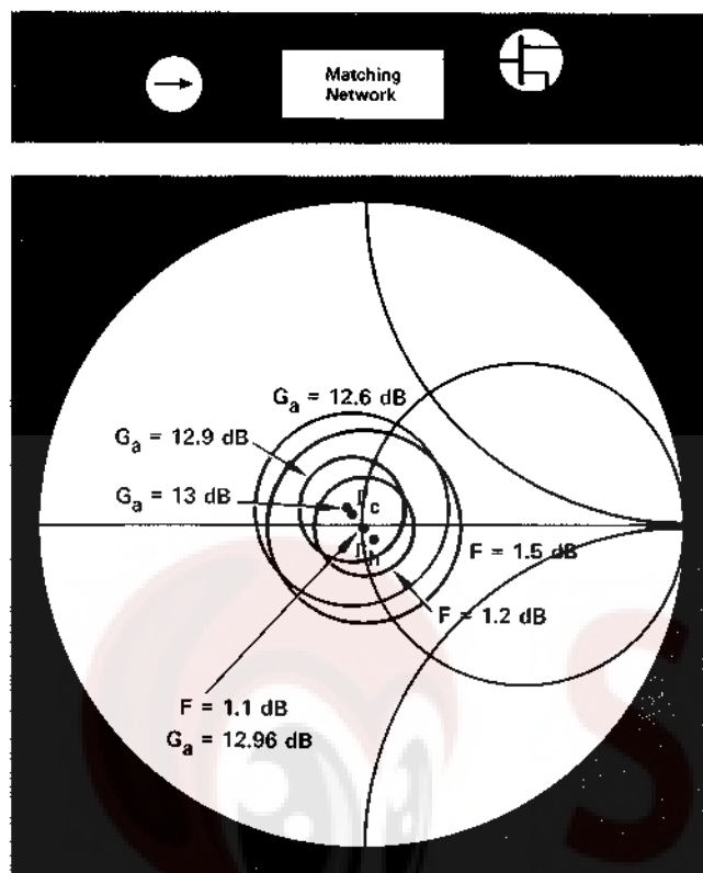
Noise figure and available gain characteristic of a 20 dB isolator, matching network, and GaAsFET.
