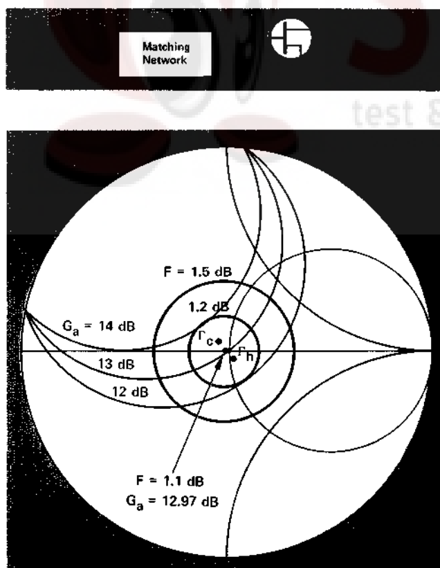
Noise figure and available gain characteristic of an amplifier stage consisting of the matching network and GaAsFET described in the text.
